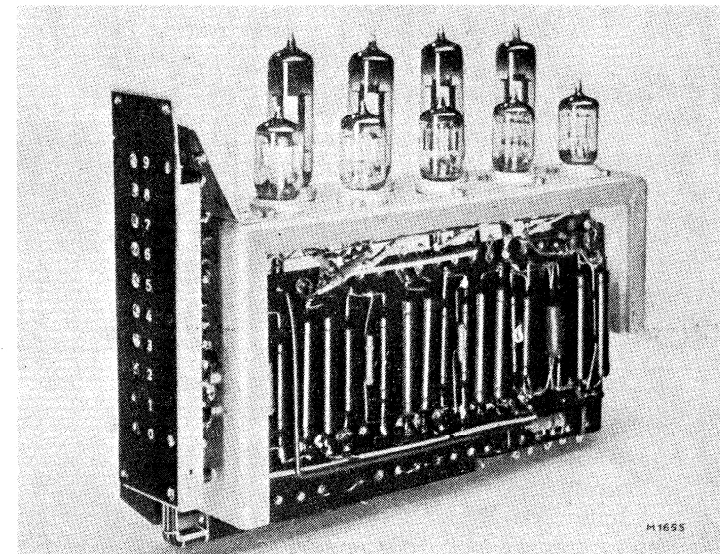
Fig. 26. Photograph of the circuits of Fig. 27.
