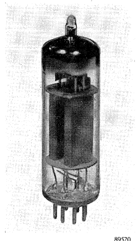
Fig. 29. Photograph of the E 29 CC.
