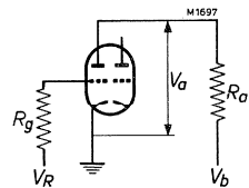
Fig. 17. Diagram for defining V_b , V_a , R_a , and R_g .
