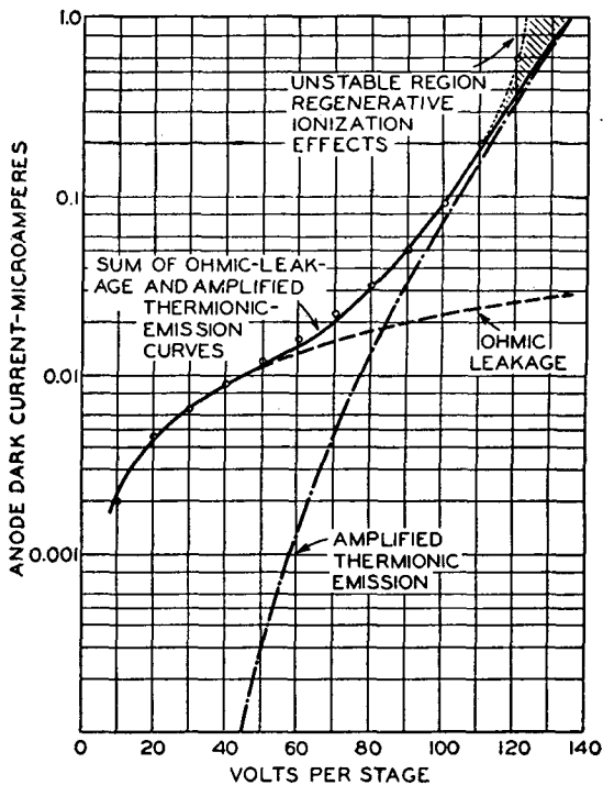
Fig. 6 — Dark current in photo-multiplier tubes.
