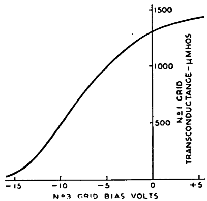
Fig. 13—Signal-grid (grid No. 1) transconductance versus oscillator-grid (grid No. 3) voltage of a typical mixer designed for use with outer-grid injection of oscillator. Signal-grid bias = -3 volts.
