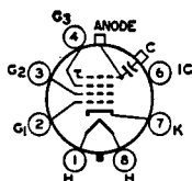
8JR ANODE = G_4 + CL FOCUSING ELECTRODE = G_3
