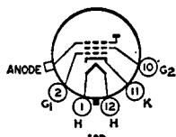
12D ANODE = G_3 + CL
