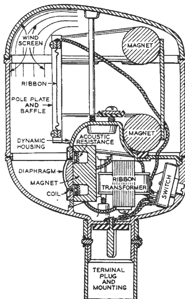
FIG. 18. Cross-sectional view of a microphone that can be used as a nondirectional, bidirectional, or cardioid microphone by turning the switch (lower right) to the proper position.
