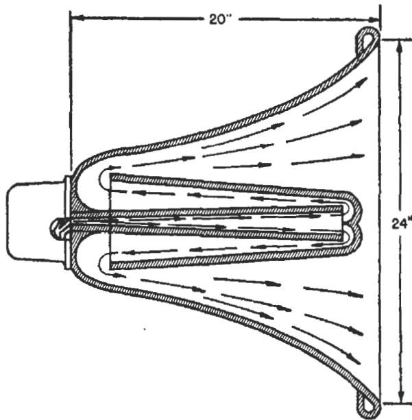
FIG. 32. Cross-sectional view of a reflex trumpet.
