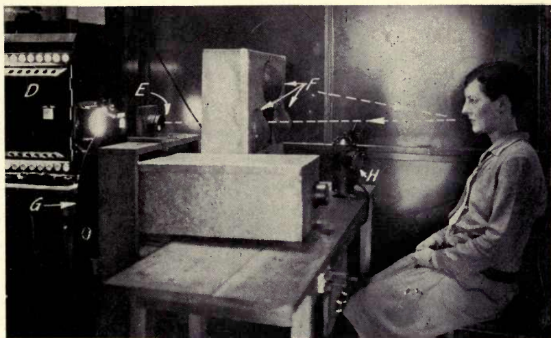
The arrangement of the scanning apparatus used at the General Electric Co., Schenectady. This is similar to the system sketched in Fig. 63. D is the light house of the arc lamp, G, the scanning disc, E the lens, F the photoelectric cell, and H the microphone. The dotted lines show the path of the scanning beam which is reflected from the face of the performer to the three sensitive photoelectric cells.
