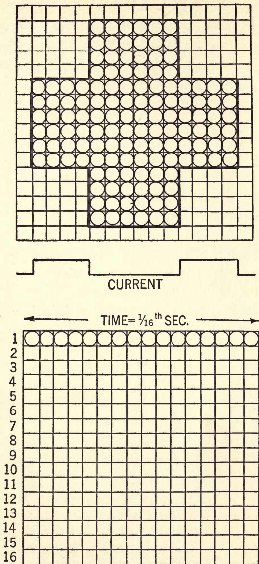
FIG. 56.—Graphic and simplified analysis of the scanning problem. This shows the number of picture units involved in the transmission of a black cross using a scanning disc with only 16 holes.
