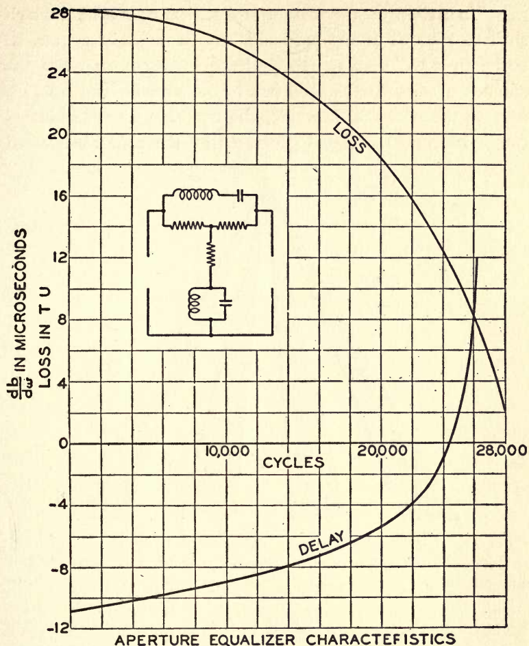
FIG. 32.—Special circuit developed for equalizing the aperture effect, its amplitude and phase characteristics. (Courtesy Bell Telephone Laboratories, Inc.)
