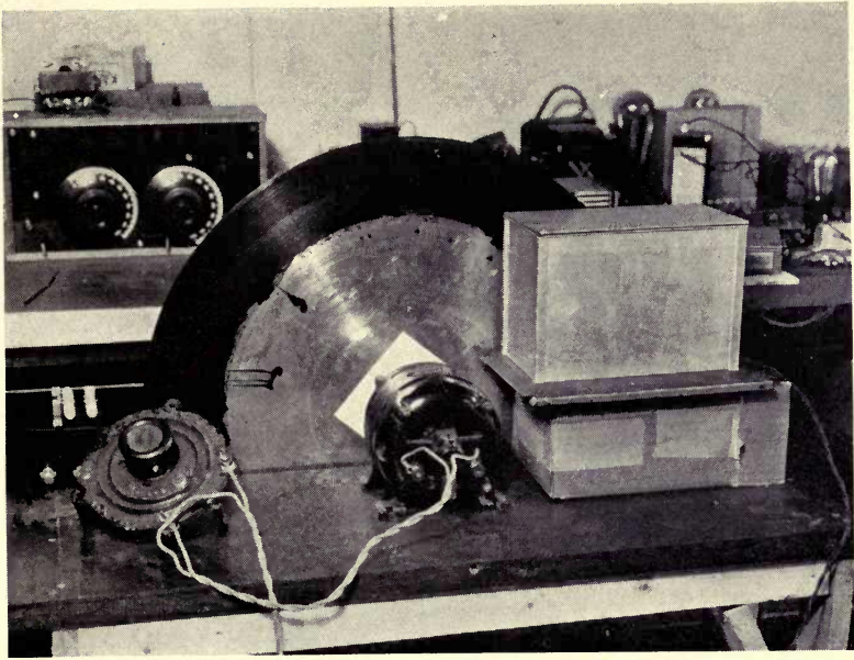
A scanning disc set up for laboratory experimenting with television. The photoelectric cell is mounted in the metal box seen at the right hand side of the photograph. The edge of the disc is coated with lamp black to prevent conflicting reflections.
