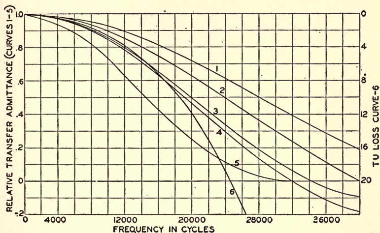
FIG. 31.—These curves illustrate in a graphic way the equivalent transfer admittance of various apertures. (Courtesy Bell Telephone Laboratories, Inc.)
