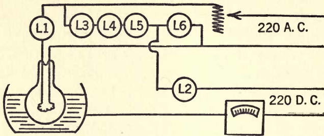
FIG. 25.—Another method of depositing sodium in the construction of photoelectric cells. The drawback of this system, as far as the amateur is concerned at least, is the necessity of having two sources of 220-volt current.
