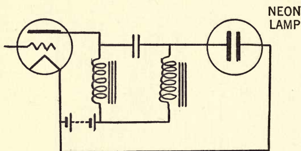
FIG. 45.—Use of two chokes and one set of B batteries in connecting a neon lamp to the output circuit of a television amplifier.
