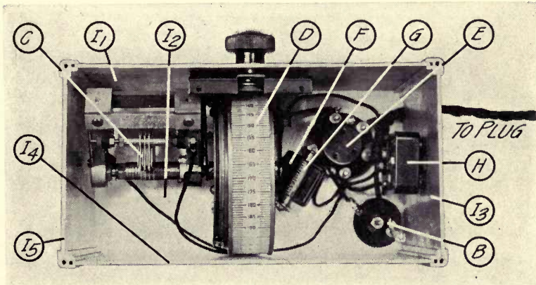
Showing the arrangement of the instruments within the short wave tuner. C is a short wave condenser, D a drum dial, G a grid leak, F a grid condenser, E a cushion socket, B a choke, and H a small variable condenser used to control the oscillations of the detector.
