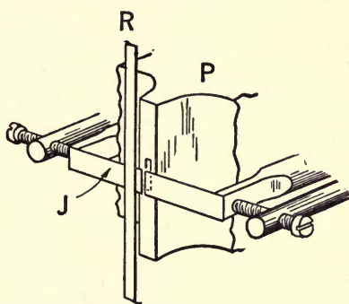
FIG. 12.—Details of the light valve used in the Bell phototelegraphic system. The ribbon R, which is arranged in the magnetic field of the magnet P, is moved slightly upon the passage of the picture current. This slight movement permits light to pass. (Courtesy Bell Telephone Laboratories, Inc.)
