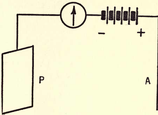
FIG. 20.—Diagrammatic representation of a photoelectric cell. The surface of P is covered with photo-active material. When light falls upon this surface, electrons are emitted and pass from P to A.
