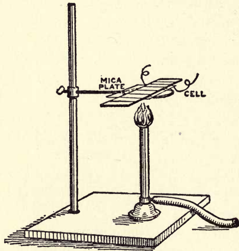
FIG. 51.—Method employed in annealing selenium used in the construction of selenium cells.
