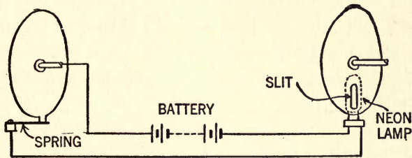
FIG. 69.—Simple indicator of synchronism. When the glow of the neon lamp is seen, this indicates that the wheel at the transmitter is running in perfect step with the wheel at the receiver.
