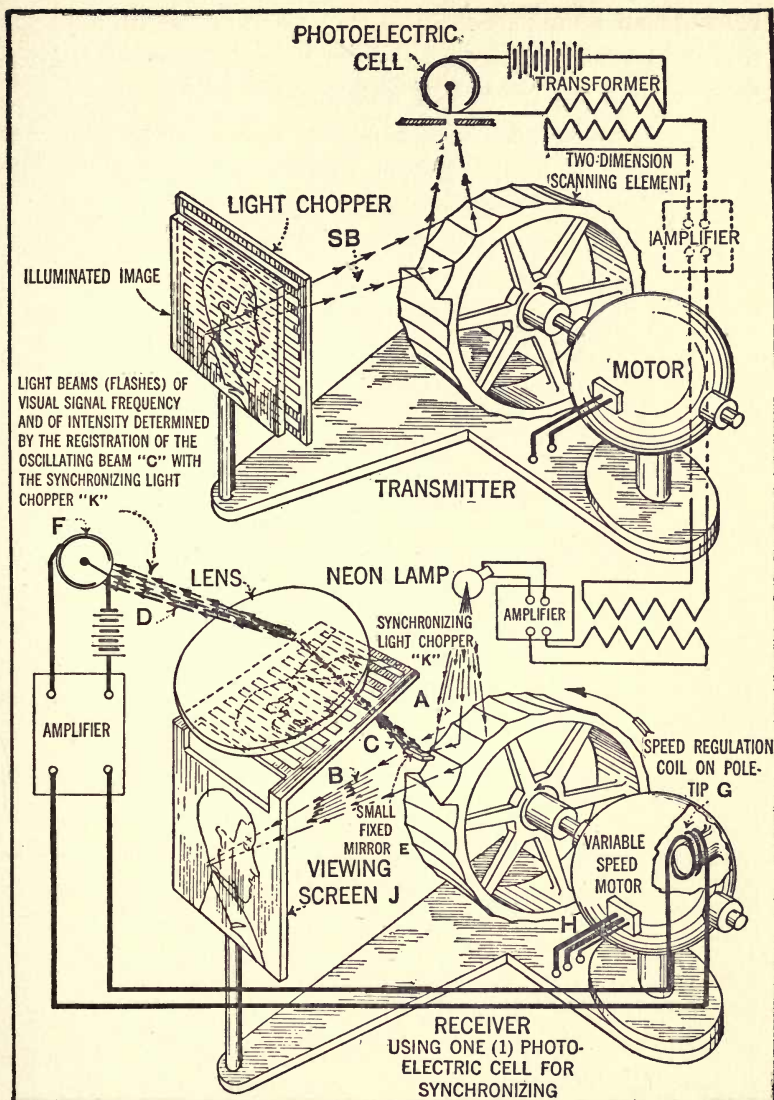
FIG. 70.—Transmitter and Receiver. The automatic synchronizing system is shown in heavy lines.
