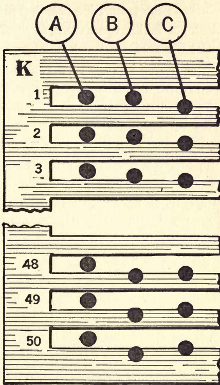
FIG. 71.—A. Successive flashes in beam from neon tube registering with successive slits in the light chopper, showing that the motor speed is too high. B. Flashes progressively overlap the chopper bars, showing speed drop from high to low. C. The flashes are partly intercepted by the bars, and half of the light passes through the slits so as to fall upon the photoelectric cell shown in Fig. 1. This condition is the ideal interception of the flashes to produce the least oscillation relative to synchronism.
