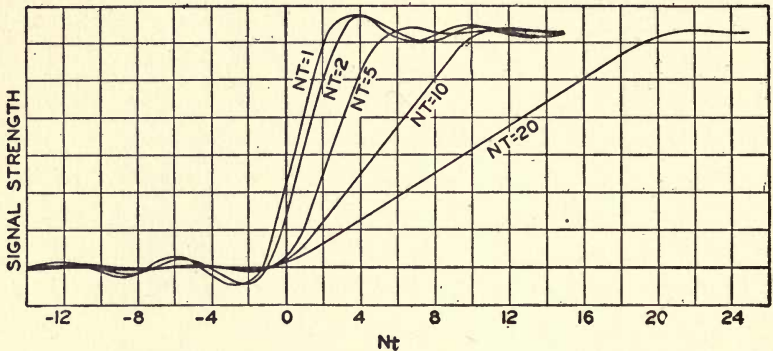
FIG. 29.—Distortion in an elementary frequency change as caused by a square aperture and ideal frequency restriction. (Courtesy Bell Telephone Laboratories, Inc.)
