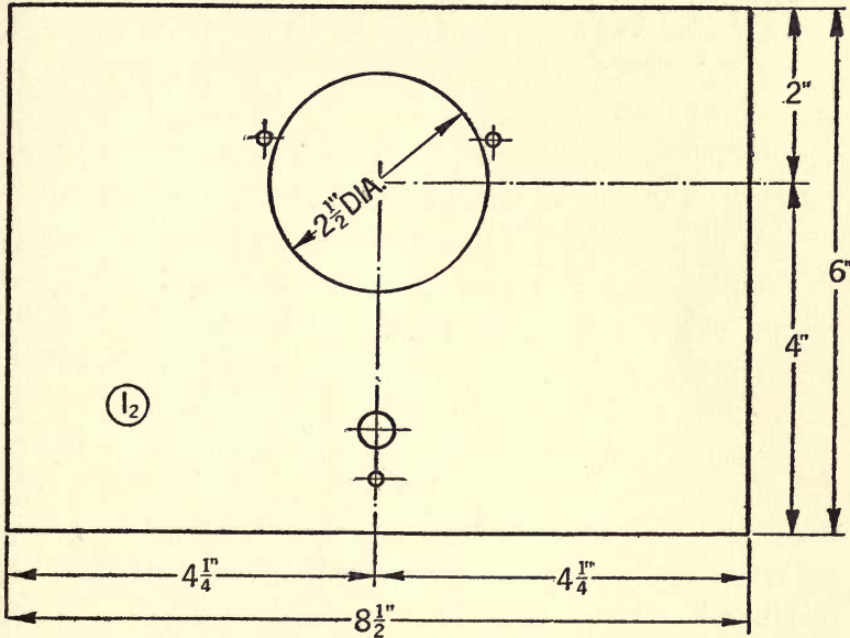
FIG. 75.—Drilling plan for the top plate of metal box for the short wave tuner.
