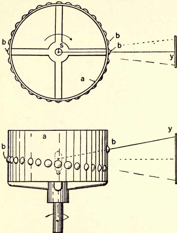
FIG. 61.—Jenkin's method of employing a drum for scanning. The lenses are mounted in spiral fashion.
