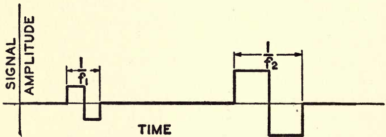
FIG. 34.—Signal detail of concentrated frequency spectrum for illustrating the effect of envelope delay. (Courtesy Bell Telephone Laboratories, Inc.)
