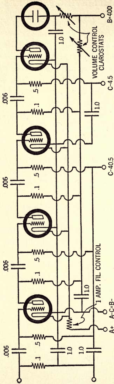
FIG. 42.—Circuit diagram of a specially designed amplifier suitable for amateur television experiments.
