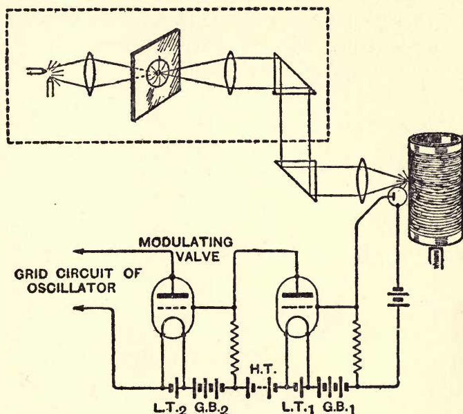
FIG. 6.—Showing the arrangement of the essential parts of the Karolus picture transmitter. The photoelectric cell is shown mounted adjacent to the picture on the revolving cylinder.
