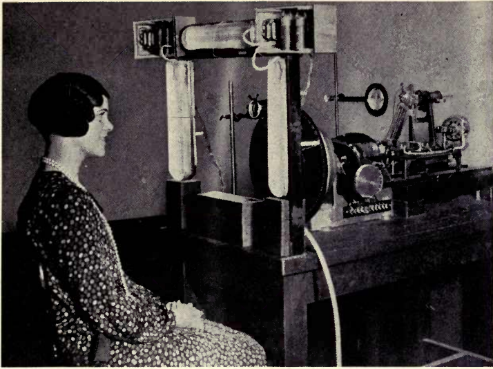
The scanning apparatus of the television transmitter designed by the engineers of the Bell Telephone Laboratories. Here a single beam is used, which after striking the face of the object or performer, as the case may be, is reflected to the three large and sensitive photoelectric cells shown mounted in the form of an arch. (Photo Courtesy Bell Telephone Laboratories, Inc.)
