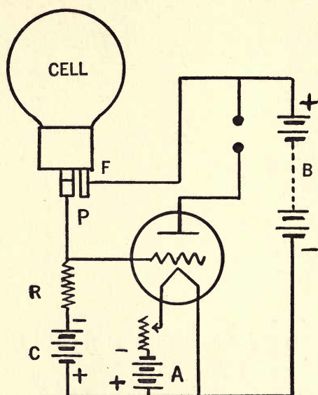
FIG. 17.—Connections for a single tube photoelectric cell amplifier. The resistance R will be found to vary, \frac{1}{2} megohm being about correct for Burt sodium cells. Other type cells will probably require higher resistances. The output of this amplifier may be fed to another amplifying system.
