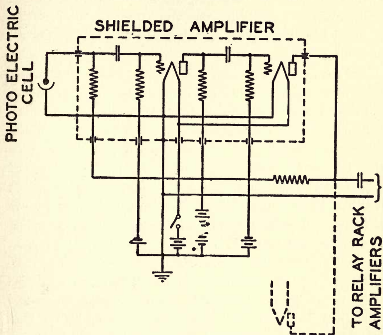
FIG. 35.—Ideal circuit of the resistance coupled type for amplification from a photoelectric cell. The dotted lines represent the copper shield about the amplifier. (Courtesy Bell Telephone Laboratories, Inc.)
