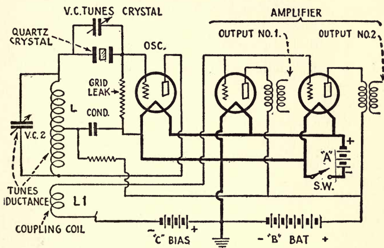
FIG. 67.—Method used in incorporating a quartz crystal in an oscillating circuit. When so placed, a crystal will actually control the frequency of oscillation. Due to this, such crystals have been successfully employed in bringing about synchronism between television receivers and transmitters. (Courtesy "Radio News.")
