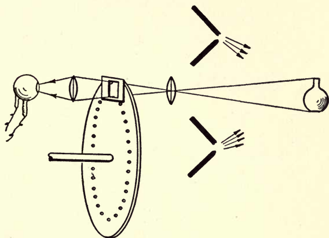
FIG. 62.—In this scanning system, the object to be transmitted is illuminated with several powerful sources of light. (Courtesy Bell Telephone Laboratories, Inc.)
