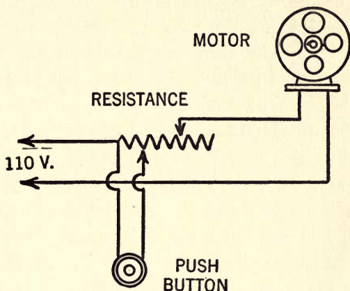
FIG. 66.—One method used to control the speed of a fractional horsepower motor with a small resistance and a push button which is constantly held in the hand of the operator. Two contacts are arranged on the resistance to enable the operator to obtain close adjustment.
