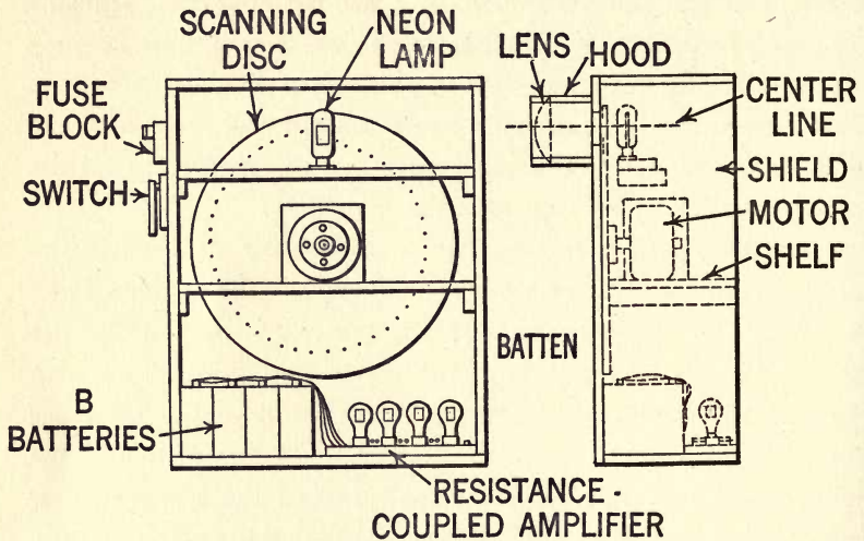
FIG. 78.—General arrangement of the parts making up a television receiver. The box is made of three-quarter-inch white pine painted black inside to prevent reflection and to sharpen the outline of the received picture.
