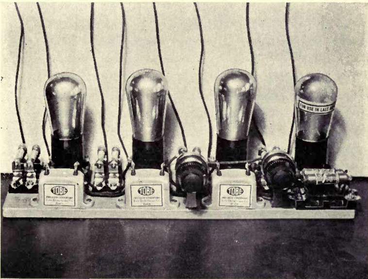
A photograph of a special resistance-coupled amplifier designed for the amplification of television signals.
