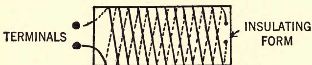
FIG. 48.—Bidwell selenium cell is constructed by winding two wires upon an insulated form. Selenium is placed between the wires.
