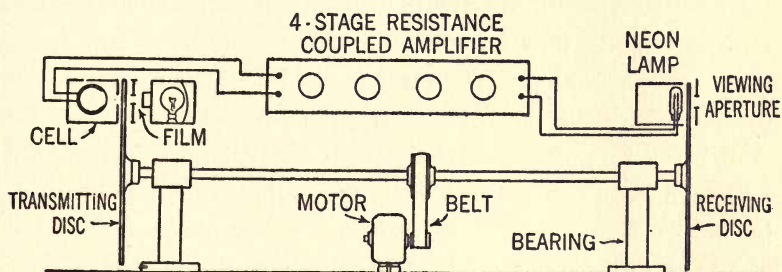
FIG. 73.—Diagram showing the simple arrangement of apparatus for a television transmitter and receiver which any experimenter may set up at home. Perfect synchronism is brought about by the simple expedient of mounting the transmitting and receiving scanning discs on the same shaft.
