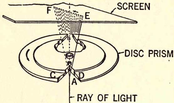
FIG. 59.—Revolving glass prism used for scanning in the Jenkins system of picture transmission. (Courtesy Q S T.)
