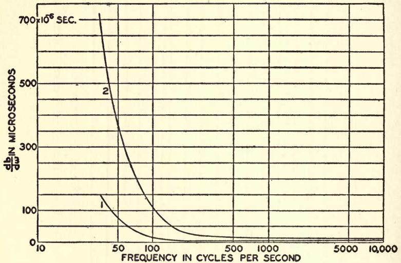
FIG. 37.—Envelope delay characteristics of (1) an output transformer and (2) a high-ratio input transformer. (Courtesy Bell Telephone Laboratories, Inc.)
