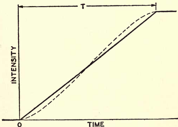
FIG. 28.—Possible distortion of an elementary signal change that might be brought about by a square aperture. (Courtesy of Bell Telephone Laboratories, Inc.)
