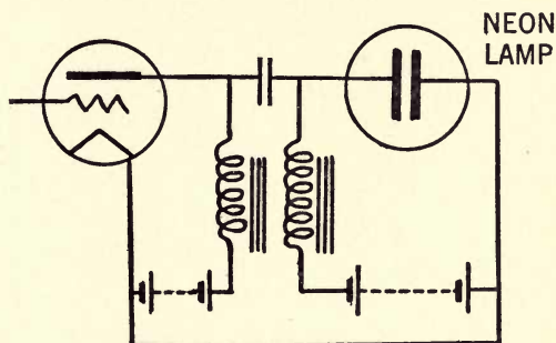
FIG. 44.—Neon lamp connected to the output circuit of vacuum tube amplifier using two impedances and two sets of B batteries.
