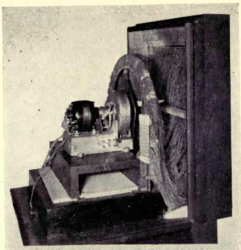
The complete high-speed distributor with its 2500 contacts and connecting wires leading to the tiny tinfoil electrodes of the special neon tube. The revolving contact arm is also driven by two motors to insure accurate synchronism. (Photo Courtesy Bell Telephone Laboratories, Inc.)
