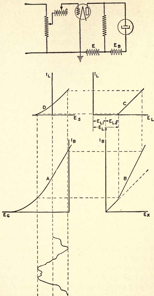
FIG. 40.—Another neon lamp circuit with curves showing operating characteristics of circuit arranged for linear operation of the lamp. (Courtesy Bell Telephone Laboratories, Inc.)
