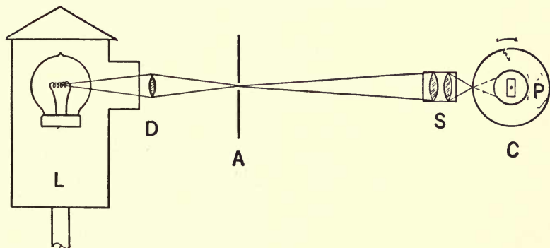
FIG. 11.—Simple elements of the Bell Telephone phototelegraphic system. L is the light house, D a condensing lens, A an aperture, S a projection lens, C the transparent cylinder, and P the photoelectric cell. (Courtesy Bell Telephone Laboratories, Inc.)
