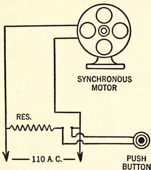
FIG. 65.—Showing the method of reducing momentarily the speed of a 60-cycle synchronous motor by inserting a resistance with a push button.
