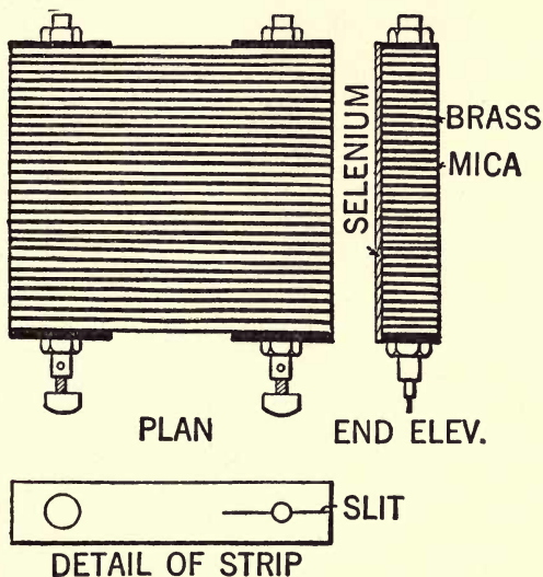
FIG. 49.—Townsend selenium shown here is made up of two separate sets of brass plates properly insulated from each other. The spaces between the plates are filled with molten selenium.
