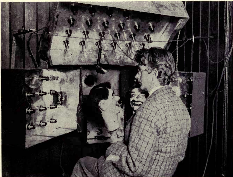
The Baird scanning mechanism. This system is similar to that illustrated in the diagram, Fig. 62. The disadvantage of this system lies in the fact that the subject has to remain exposed to a powerful source of illumination.
