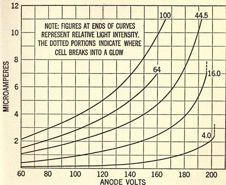
FIG. 23.—Gas-filled photoelectric cell performs differently than a vacuum type of cell. These volt-ampere curves will emphasize this fact. These curves were plotted by the aid of the apparatus illustrated in Fig. 21.
