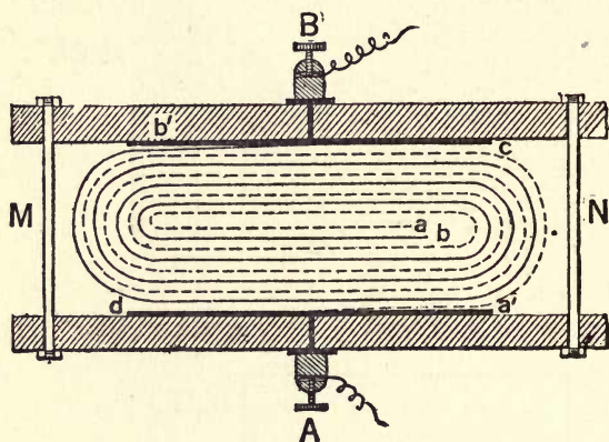
FIG. 50.—Mercadier selenium cell is made by winding together two strips of brass, the stripes being separated by a third strip of insulating material.
