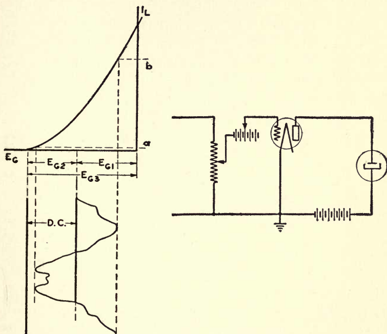
FIG. 39.—Circuit diagram and operating characteristic of a neon lamp amplifier. (Courtesy Bell Telephone Laboratories, Inc.)
