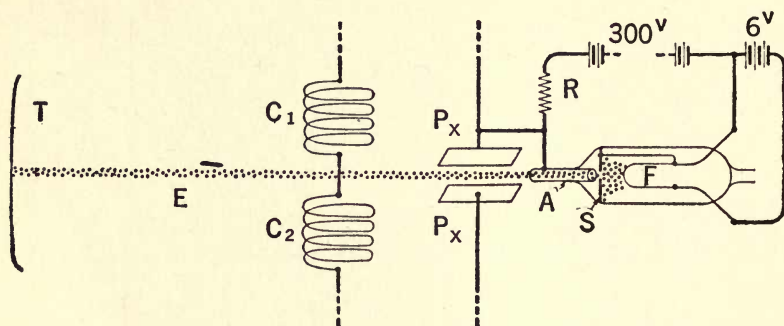
FIG. 3.—Schematic layout of the necessary components of a cathode ray tube used to make visible oscillating currents. The electron stream created by the hot filament F is forced out of its normal path by charges on the plates P_x and by currents in the coils C_1 and C_2 . The electron stream produces a visible effect on the screen T. This principle has been applied to the reproduction of television pictures.
