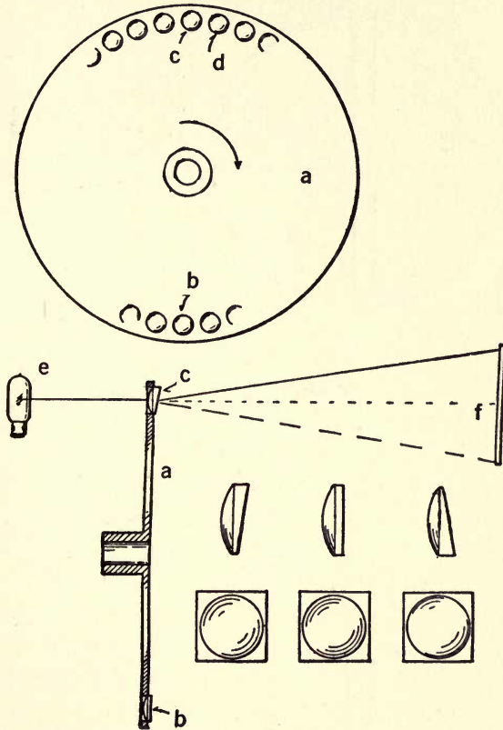
FIG. 60.—Jenkins' scanning discs using lenses ground in forms between the extremes shown in the lower right hand corner of the diagram.
