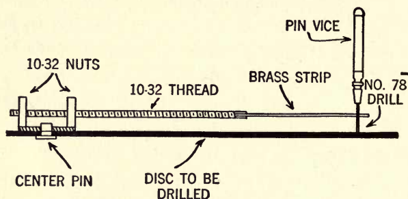
FIG. 64.—Drilling jig used in accurately locating and drilling the holes in scanning discs. This jig takes advantage of the fact that a 10-32 screw thread causes a rod to advance .015 of an inch for every half revolution.
