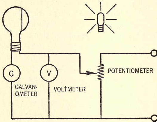
FIG. 21.—The simple circuit used to determine the volt-ampere characteristics of a cell. Such characteristics are plotted in the curves illustrated in Figs. 22 and 23. The potentiometer is naturally connected across a source of voltage, which as one of the curves shows, may go as high as 220.
