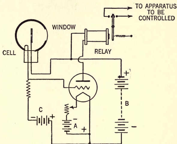
FIG. 18.—How a photoelectric cell is used to control a relay. When used in this manner, a cell will cause a beam of light to operate large machines like electric motors, horns or bells. If more stages of amplification are used, a less sensitive relay may be employed.
