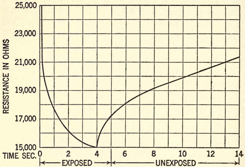
FIG. 46.—This curve was taken to show the lag of selenium in returning to its point of normal or "dark resistance" after being exposed to a source of light.
