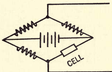
FIG. 47.—Korn method of connecting a selenium cell in one arm of a wheatstone bridge to overcome the lag of the cell.
