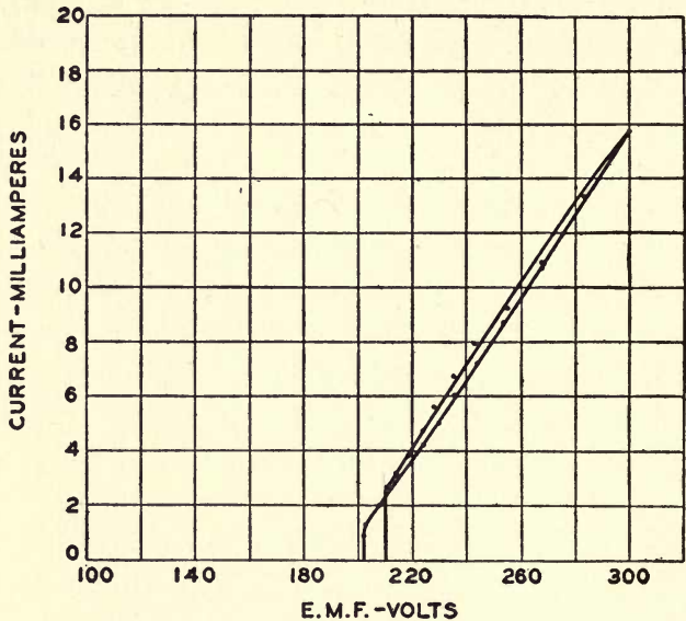
FIG. 38.—Current-voltage characteristic curve of an ordinary neon lamp similar to the types now used for television illumination. (Courtesy Bell Telephone Laboratories, Inc.)
