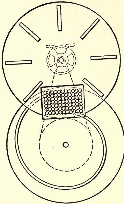
FIG. 58.—Scanning system first employed by the English television experimenter, Baird. As will be seen, Baird used a continuous spiral, the light being moulded into round beams by means of a cellular structure made up of round metal tubes.
