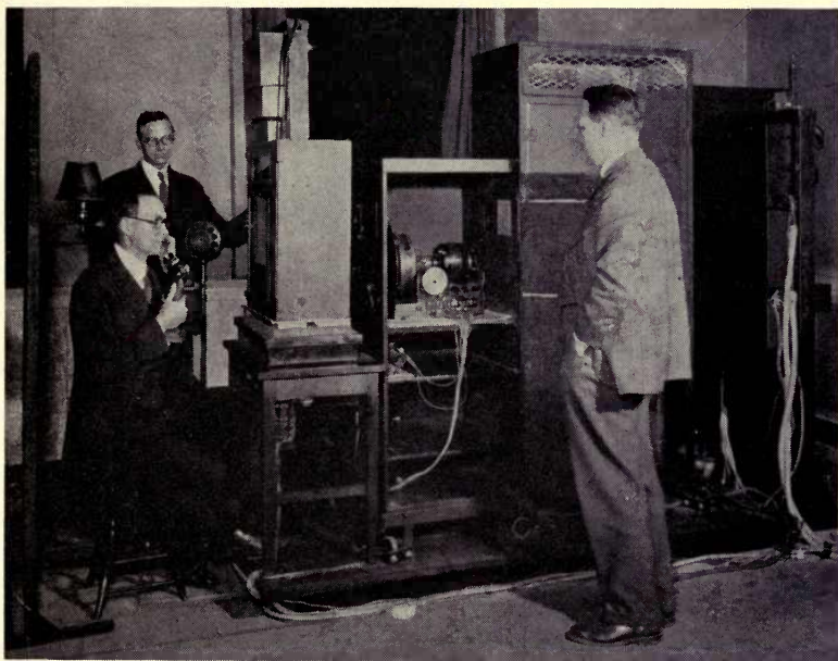
The television transmitter developed by the Bell Telephone Laboratories, Inc. This is perhaps the most perfect device of its kind in the world today. The man with the telephone sits before the scanning apparatus. Three ultra-sensitive photoelectric cells are mounted within the cabinet before him. The motor driving the scanning disc may be seen mounted in the second cabinet to the right. (Photo Courtesy Bell Telephone Laboratories, Inc.)
