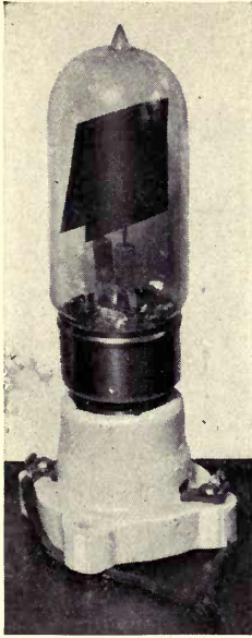
A special neon lamp with electrodes measuring 1\frac{1}{2} \times 1\frac{1}{2} . Such lamps are connected in the output circuits of television receivers.
