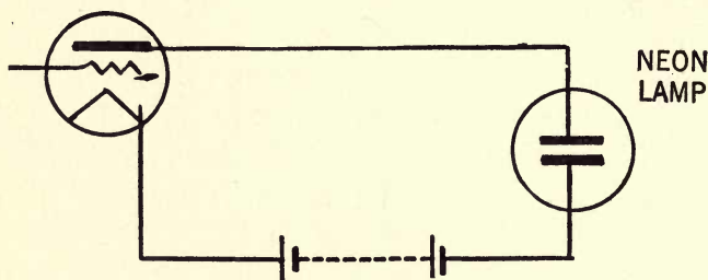
FIG. 43.—One way of connecting a neon lamp of a television receiver to the last or output tube of an amplifier. The plate voltage of the last tube should be larger than the striking voltage of the neon lamp.
