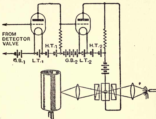
FIG. 7.—The essentials of the Karolus picture receiving system. The Kerr cell, which automatically regulates the intensity of the light beam to correspond with the fluctuations at the transmitter, is shown connected to the output of the vacuum tube amplifier. The cylinder carries the photo-sensitive paper upon which the picture is to be placed.
