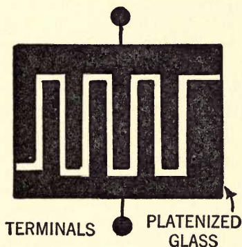
FIG. 52.—Wein selenium is constructed from a platinized piece of glass, the electrodes being formed by separation of the platinum surface into two parts. A thin film of selenium occupies the space between the two surfaces.
