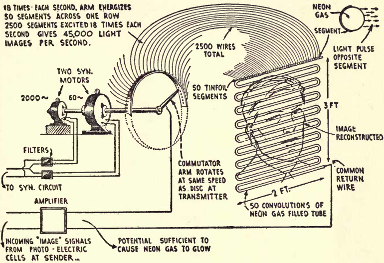
FIG. 2.—Showing the method used in impressing impulses upon a great neon tube provided with 2500 electrodes and a revolving contactor which properly distributes the light changes to the electrodes in such a way as to create the picture illusion. (Courtesy "Radio News.")
