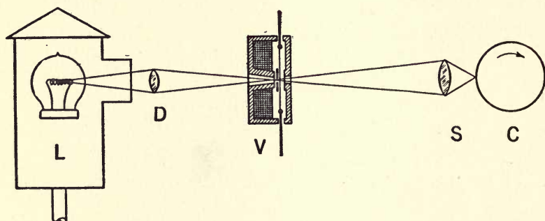
FIG. 13.—Principal parts of the Bell picture receiver. L is the light house, D a condensing lens, V the light valve, S a condensing lens and C the cylinder carrying the photo-sensitive paper. (Courtesy Bell Telephone Laboratories, Inc.)
