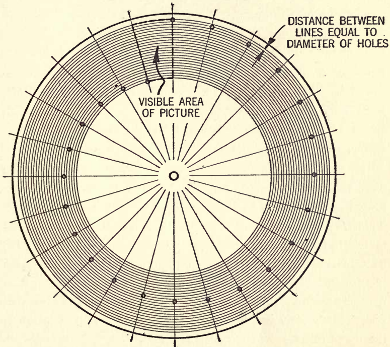
FIG. 53.—Simple way of laying out a television scanning disc for drilling. By this method the spiral automatically develops, its formation requiring no elaborate measuring instrument or involved formula.
