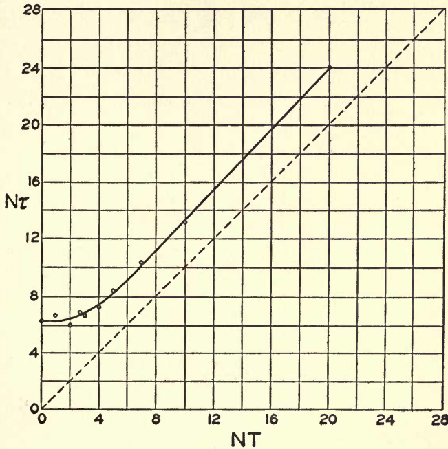
FIG. 30.—How sluggishness may be caused by distortion as a function of the aperture width and frequency restriction. (Courtesy Bell Telephone Laboratories, Inc.)
