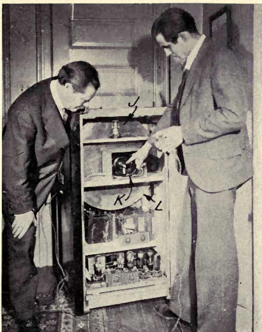
The inside of the Alexanderson television receiver. J points out the neon tube, K the synchronous motor and L the scanning disc. A powerful audio-frequency amplifier of special design is placed in the bottom of the cabinet.
