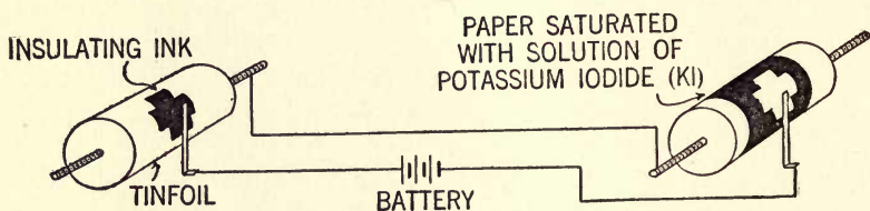
FIG. 5.—Diagram of a very simple picture transmitter similar to the first one employed by Bain in 1842. The picture to be transmitted is first drawn with insulating ink upon a metal cylinder. A contact riding over this cylinder causes the circuit to open every time the contact reaches this ink. This is recorded at the receiver by the action of a chemical when electrolyzed.
