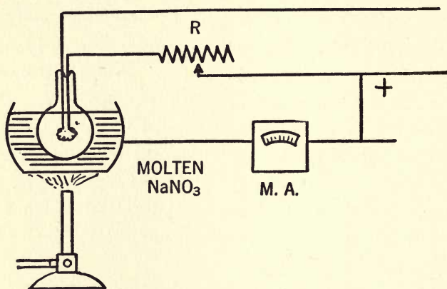
FIG. 24.—Electrolyzing sodium nitrate to deposit pure sodium upon the inside of a glass tube. It is this process that is employed in the manufacture of the Burt photoelectric cell. Such a process produces an extremely pure surface of the metal inside the cell. The milli-ammeter is included in the circuit to indicate the progress of the deposition.
