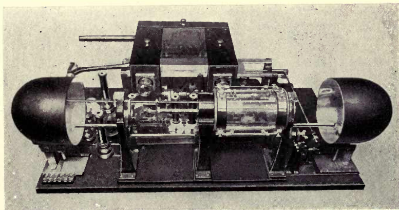
The transmitter of the Ranger system. As in all other photo-telegraphic systems, the picture is progressively explored with a fine pencil of light.
