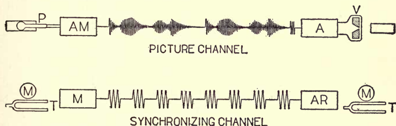
FIG. 14.—Diagrammatic representation of the picture and synchronizing currents used in the Bell phototelegraphic system. (Courtesy Bell Telephone Laboratories, Inc.)
