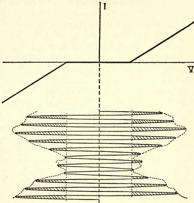
FIG. 41.—Diagrammatic representation of the relation between modulated high frequency wave impressed on grid type neon lamp and lamp characteristics. The intensity of the glow is proportional to the shaded area. (Courtesy Bell Telephone Laboratories, Inc.)
