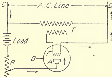
FIG. 46.—Scheme of Connections for using Tungsar Rectifying Valve to Rectify a Low-frequency Alternating Current.
