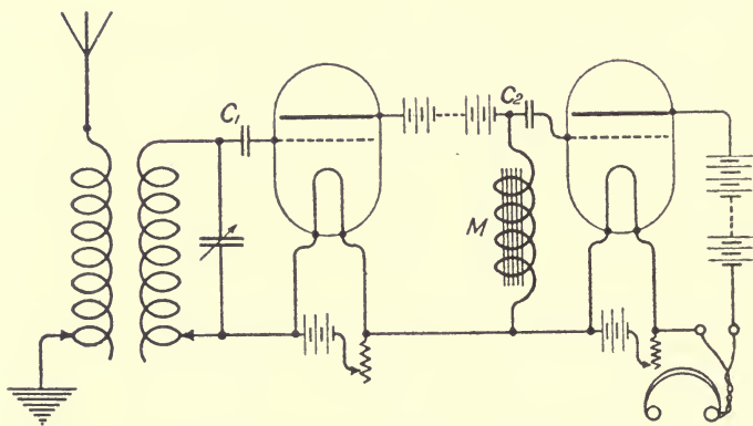
FIG. 132.—Receiving arrangement of two Valves coupled through an Iron-cored Choker, due to Mr. A. Hoyt Taylor.
