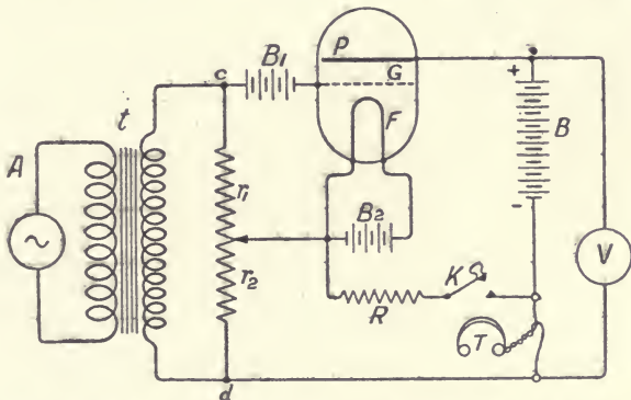
FIG. 142.—Method of J. M. Miller for Measuring the Amplification Factor \mu and internal resistance of a Thermionic Valve.
