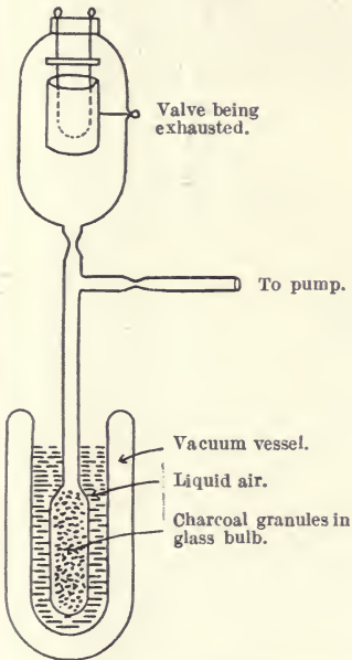
FIG. 53.—Sir James Dewar's method of making a High Vacuum by the Absorption effected by Charcoal cooled in Liquid Air.
