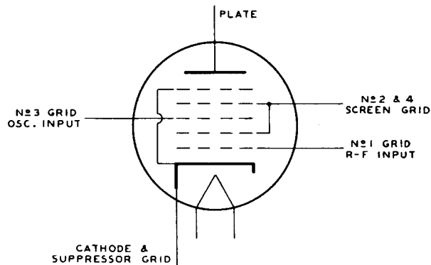
Fig. 4 - Outer-grid-injection mixer (6L7).
