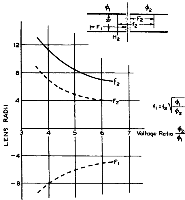
Fig. 15 - Focal length and position of focal points of cylinder as function of voltage ratio (after Epstein, reference 16).
