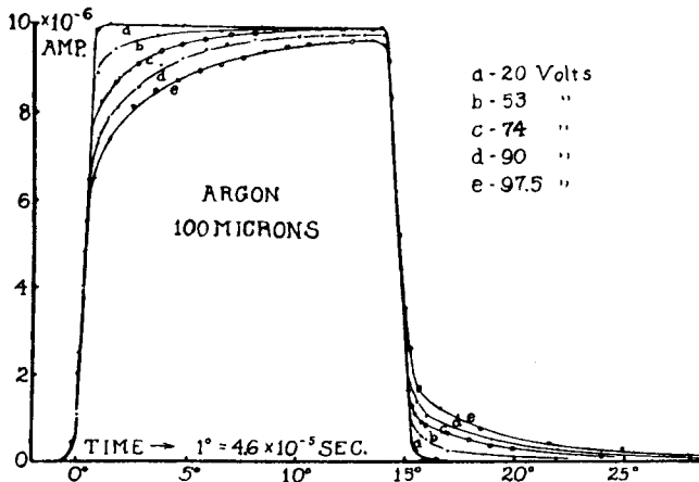
Fig. 14 - Time-lag plots for an argon cell at 100 microns of pressure.
