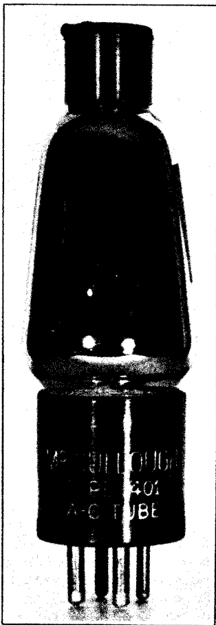
Fig. 17 - McCullough tube type with indirectly heated cathode.
