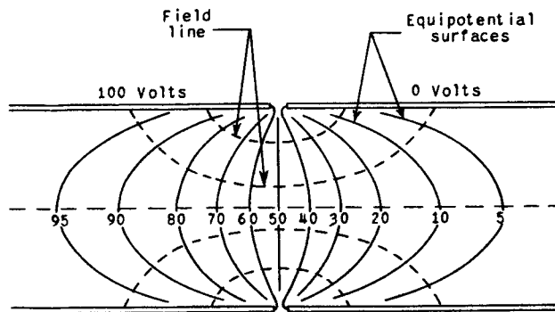
Fig. 2 - Potential distribution between two cylinders.
