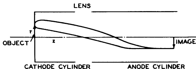
Fig. 17 - Cathode lens.
