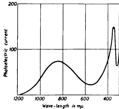
Fig. 20 - Representative spectral distribution curve of a Ag: Cs 2 O, Ag-Cs cathode with a surplus of Ag in the layer. S. Asao, Physics, 2, p. 19 (1932). Courtesy of American Physical Society.
