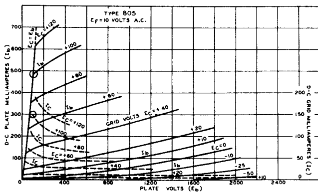
Fig. 12 - Plate and grid family for illustrating concept of plate perveance (G) in a triode for which
