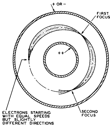
Fig. 11 - Focusing with the electrostatic field of concentric cylinders.
