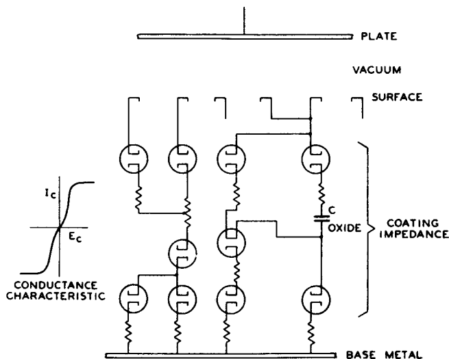
Fig. 4a - Representative diode network.
