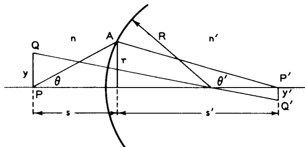
Fig. 3 - Refraction at a curved surface.
