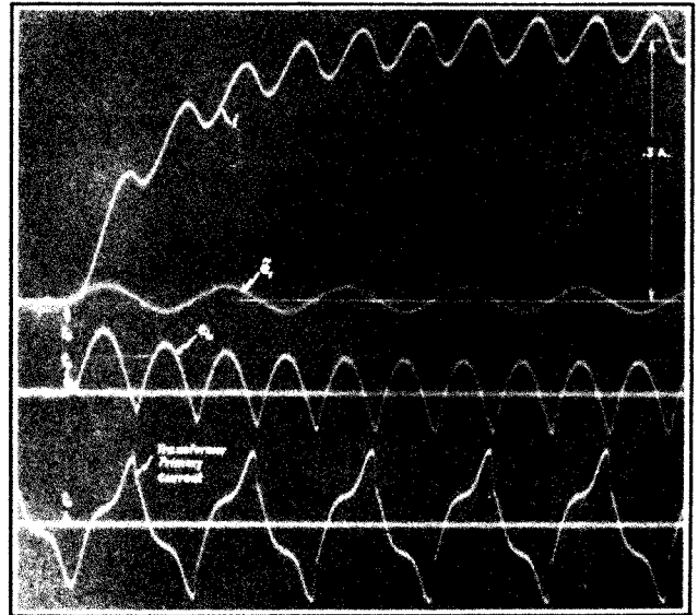
Fig. 10 - Oscilloscope taken with circuit values in Fig. 9.
