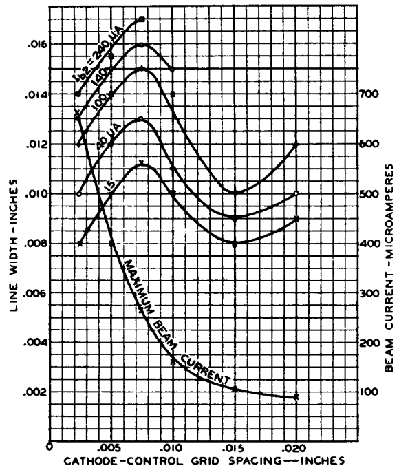
Fig. 8 - Variation of scanned line width with cathode-to-control-grid spacing.
