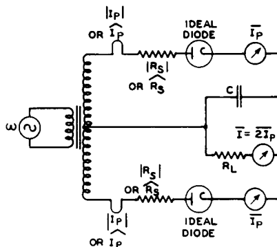
FULL-WAVE CIRCUIT
