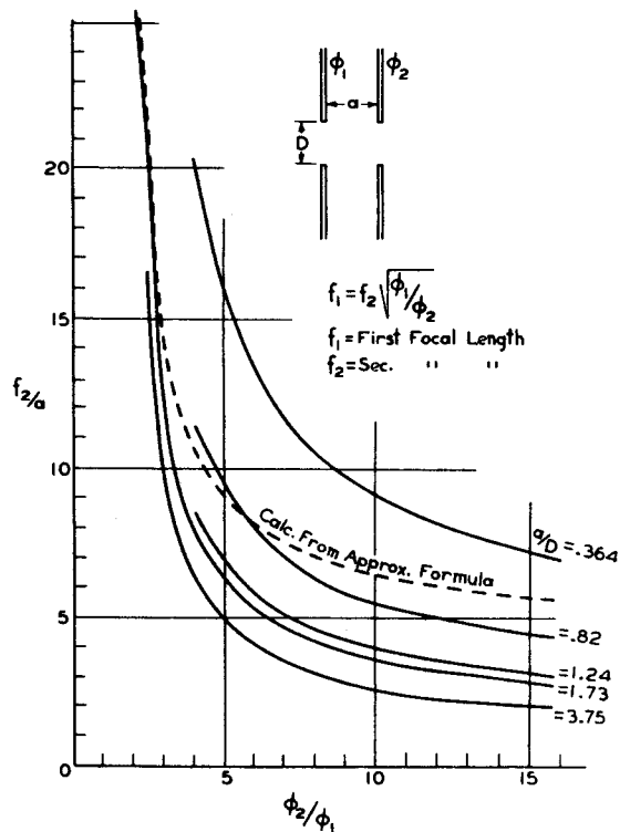
Fig. 16 - Focal length of double-aperture lenses (after Polotovski, reference 15).
