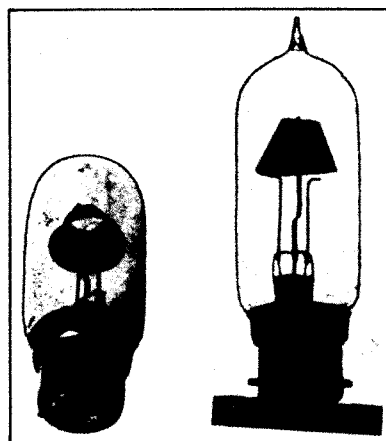
Fig. 2 - One type of Fleming valve.
