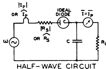
HALF-WAVE CIRCUIT
