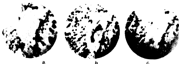
Fig. 8 - Electron emission pictures of a barium coated nickel surface. (a) Photoelectric before heating. (b) Thermionic. (c) Photoelectric after heating.
