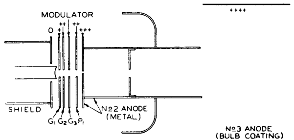
Fig. 6 - Projection-type electron gun.
