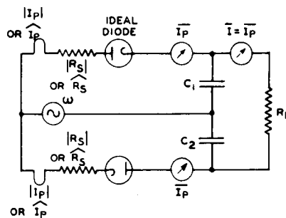
VOLTAGE-DOUBLING CIRCUIT
