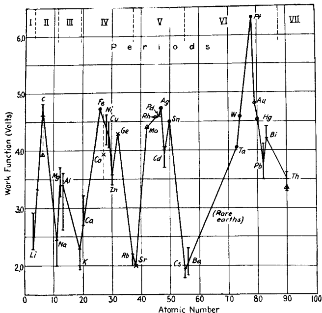
Fig. 5 - Variation of photoelectric work function throughout the periodic table. \odot , values for clean surfaces. \times , single values of uncertain precision. \Delta , reliable thermionic value (indicated only when photoelectric value is uncertain. \square , vertical lines indicate approximate range covered by various reported values.
