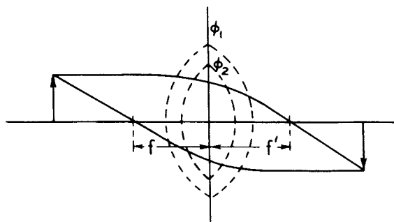
Fig. 8 - Doubler-layer lens.
