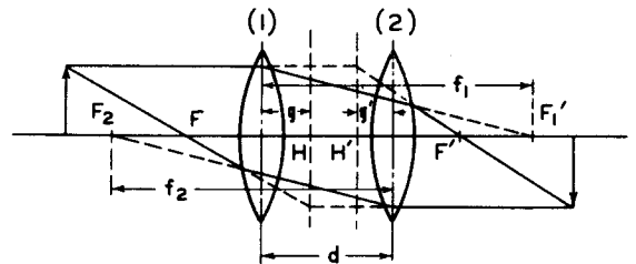
Fig. 6 - Cardinal points of a pair of thin lenses.
