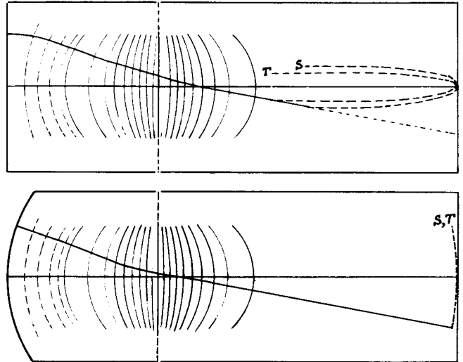
Fig. 12 - Potential distribution and image curvature in tubes with flat and curved cathode (Schematic).
