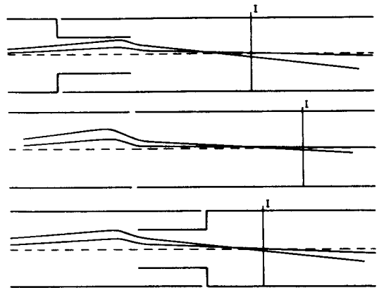
Fig. 9 - Aperture defect for cylinder lenses.
